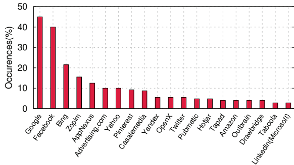
Figure 7: Top-20 trackers (grouped based on organization) and their coverage in persona pages. For example, all the Google-owned domains, such as Doubleclick, Googleapis, Google-Analytics, are grouped under the “Google” label.
