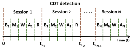
Figure 4: Timeline of phases for CDT measurement. M_i : mobile training time t_{train} + testing time t_{test} ; B_i(A_i) : desktop testing time t_{test} before (after) mobile phase; W : wait time ( t_{wait} ); R : rest time ( t_{rest} ); t_{s_i} : time of session i .
