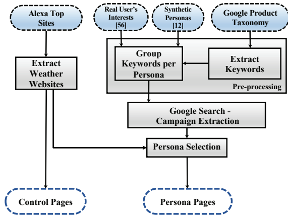
Figure 3: Persona design and automatic generation.
