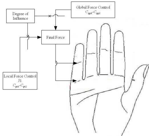
Fig. 1. The two control levels for the hand. Global force applies to all joints in the fingers, while local is specific to one joint. The degree of influence scales appropriately each level of control, and sends the final force command to the controller of the robot's hand.
