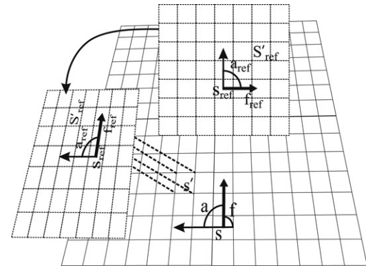
Fig. 2. Translation and rotation of the reference POMDP transition probabilities matrix.
